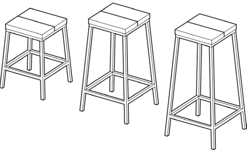
Stool 450 | 650 | 750h 290w x 290d
