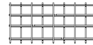
LNK400-9x15-001 Link Display Unit – 1505H x 3288W x 440D 3 shelf layers and top panel
