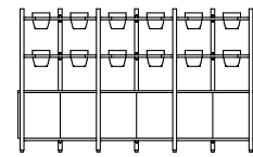
LNK400-7x15-003 Link Display Unit – 1505H x 2488W x 440D Base cabinets and 12 planters
