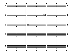
LNK400-7x19-001 Link Display Unit – 1900H x 2488W x 440D 4 shelf layers and top panel
