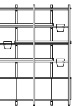
LNK400-5x23-003 Link Display Unit – 2295H x 1688W x 440D Base cabinets, 3 shelf layers, top panel and 5 planters
