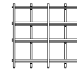
LNK400-5x15-001 Link Display Unit – 1505H x 1688W x 440D 3 shelf layers and top panel
