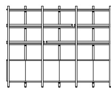
LNK400-7x19-002 Link Display Unit – 1900H x 2488W x 440D Base cabinets, 2 shelf layers and top panel
