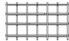
LNK400-7x15-001 Link Display Unit – 1505H x 2488W x 440D 3 shelf layers and top panel
