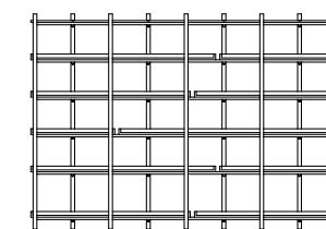
LNK400-9x23-001 Link Display Unit – 2295H x 3288W x 440D 5 shelf layers and top panel
