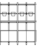
LNK400-5x19-003 Link Display Unit – 1900H x 1688W x 440D Base cabinets, 1 shelf layer, top panel and 4 planters
