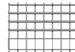
LNK400-9x23-002 Link Display Unit – 2295H x 3288W x 440D Base cabinets, 3 shelf layers and top panel
