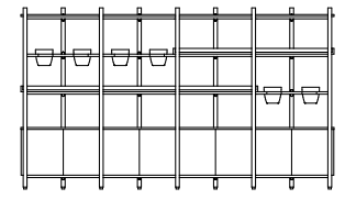
LNK400-9x19-003 Link Display Unit – 1900H x 3288W x 440D Base cabinets, 1 shelf layer, top panel and 6 planters
