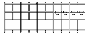
LNK400-11×15-003 Link Display Unit – 1505H x 4088W x 440D Base cabinets, 2 shelf layers and 4 planters
