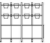
LNK400-5x15-003 Link Display Unit – 1505H x 1688W x 440D Base cabinets and 8 planters
