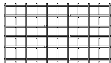
LNK400-11×23-001 Link Display Unit – 2295H x 4088W x 440D 5 shelf layers and top panel
