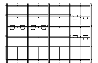
LNK400-9x23-003 Link Display Unit – 2295H x 3288W x 440D Base cabinets, 3 shelf layers, top panel and 8 planters
