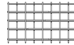
LNK400-9x19-001 Link Display Unit – 1900H x 3288W x 440D 4 shelf layers and top panel
