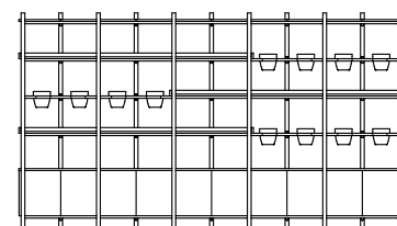
LNK400-11×23-003 Link Display Unit – 2295H x 4088W x 440D Base cabinets, 3 shelf layers, top panel and 12 planters
