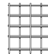
LNK400-5x19-001 Link Display Unit – 1900H x 1688W x 440D 4 shelf layers and top panel
