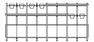
LNK400-9x15-003 Link Display Unit – 1505H x 3288W x 440D Base cabinets, 2 shelf layers and 6 planters
