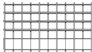
LNK400-11×23-002 Link Display Unit – 2295H x 4088W x 440D Base cabinets, 3 shelf layers and top panel
