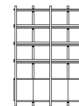
LNK400-5x23-002 Link Display Unit – 2295H x 1688W x 440D Base cabinets, 3 shelf layers and top panel
