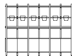
LNK400-7x19-003 Link Display Unit – 1900H x 2488W x 440D Base cabinets, 1 shelf layer, top panel and 6 planters
