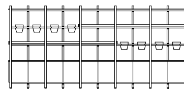
LNK400-11×19-003 Link Display Unit – 1900H x 4088W x 440D Base cabinets, 2 shelf layers, top panel and 8 planters
