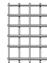
LNK400-5x23-001 Link Display Unit – 2295H x 1688W x 440D 5 shelf layers and top panel
